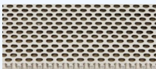
3070 OA 40.4% 3t x \phi 2 x 3mm centers
