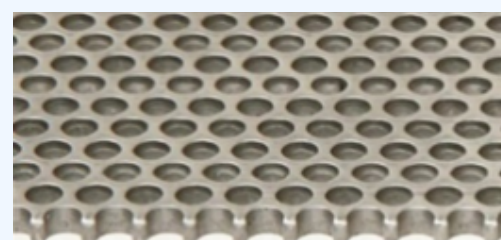
3090 OA 51.0% 3t x \phi 3 x 4mm centers
