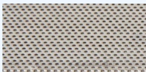
3010 OA 22.6% 1t x \phi 0.75 x 1.5mm centers
