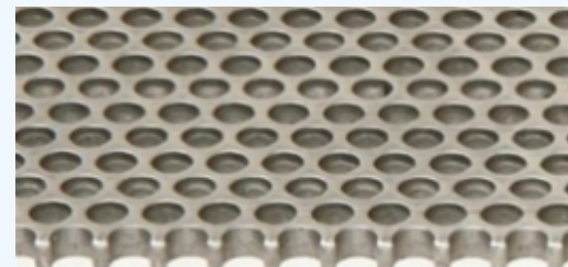
3090 OA 51.0% .1181"t x \phi .1181 x .1575" centers
